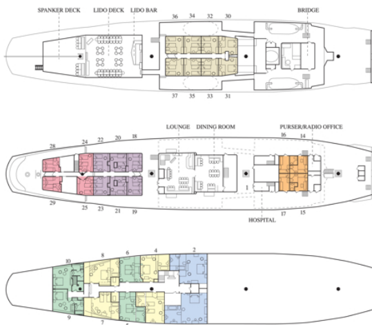
CAPTAIN'S AND LIDO DECK
