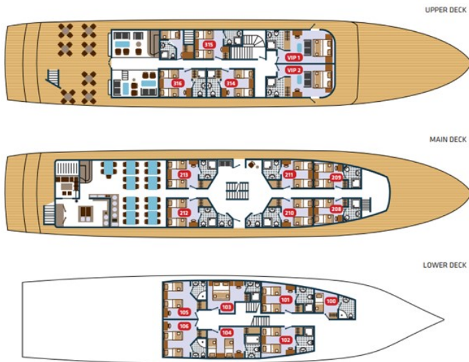
Main Deck
